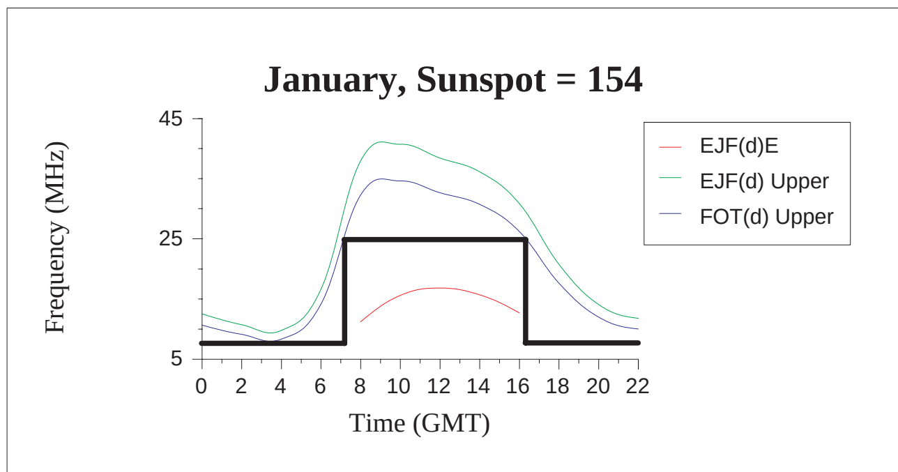
Figure 7 - Graph of January, sunspot = 154
