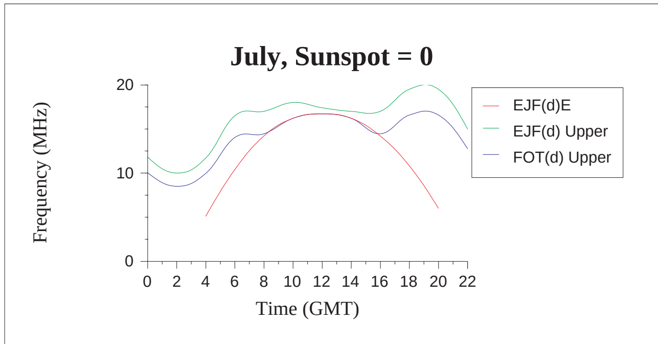
Figure 2 - Graph of July, sunspot = 0
