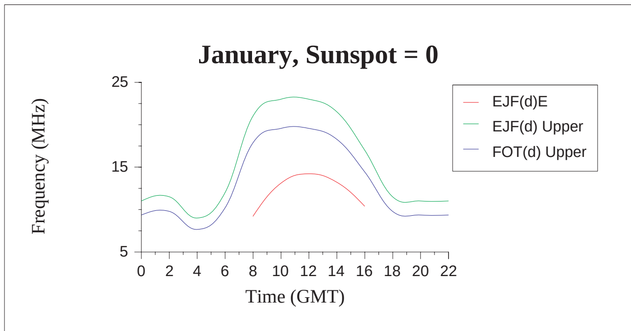
Figure 5 - January, sunspot = 0
