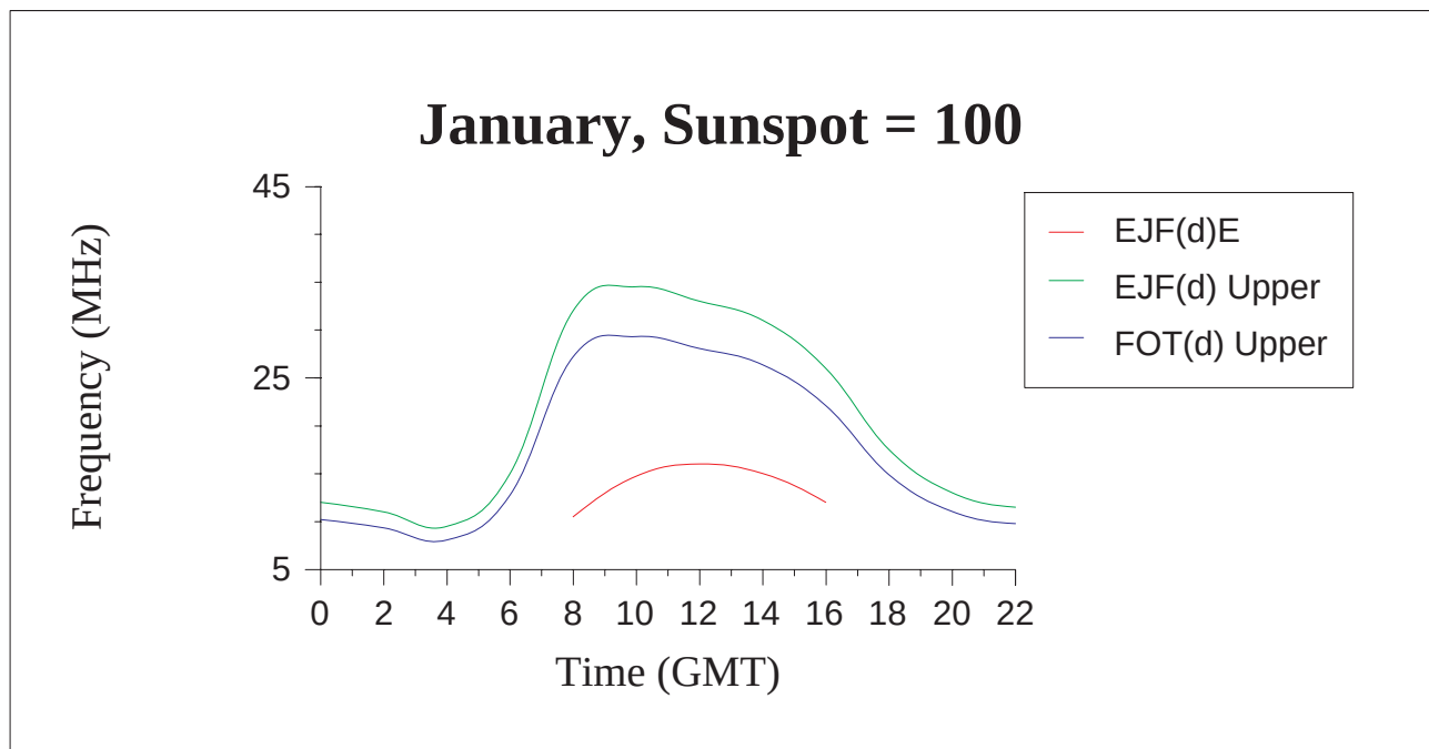
Figure 6 - Graph of January, sunspot = 100
