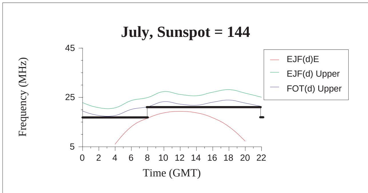
Figure 4 - Graph of July, sunspot = 144
